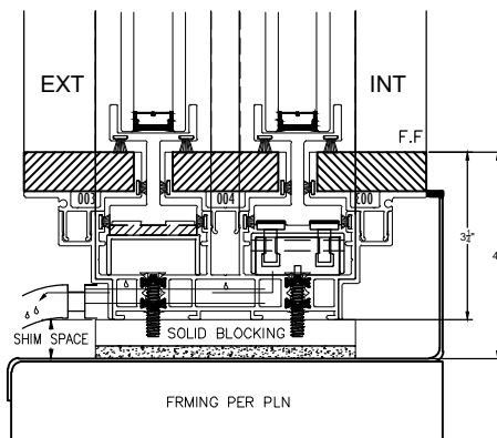
DRAINAGE DETAIL OPTION A HIDDEN TRACK
