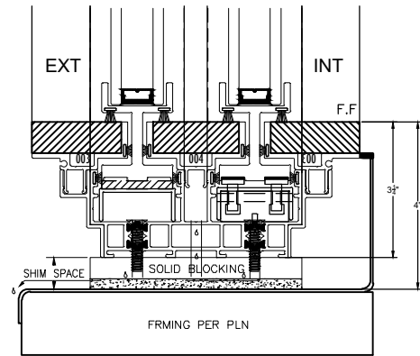
DRAINAGE DETAIL OPTION B (STANDARD) HIDDEN TRACK
