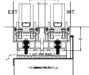
DRAINAGE DETAIL OPTION B (STANDARD)
