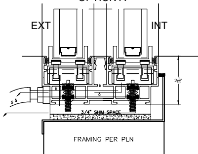
DRAINAGE DETAIL OPTION A
