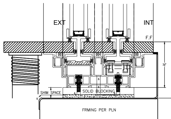
DRAINAGE DETAIL OPTION C HIDDEN TRACK
