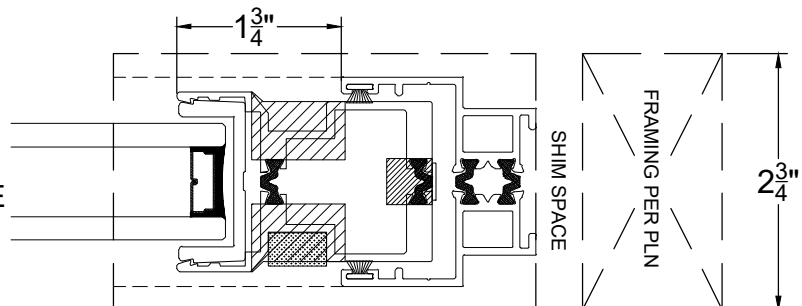
2 FLUSH POCKETING HANDLE
