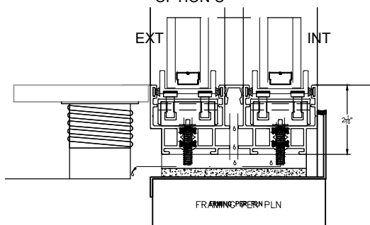
DRAINAGE DETAIL OPTION C
